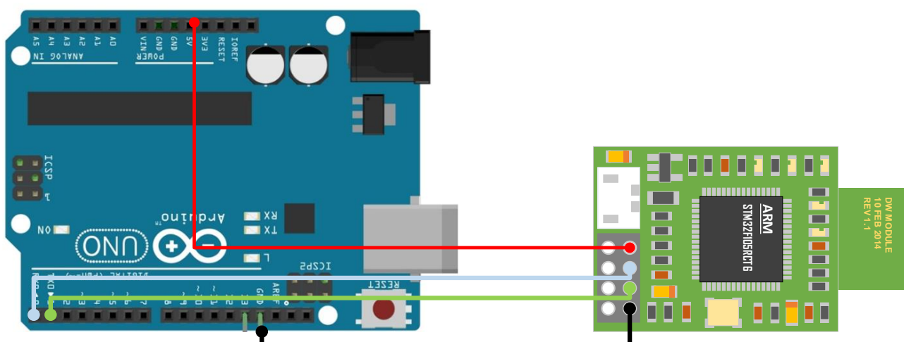
Figure 1.2 UWB Mini 3 module is connected to UNO R3
